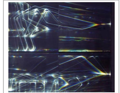
Electric Waves
